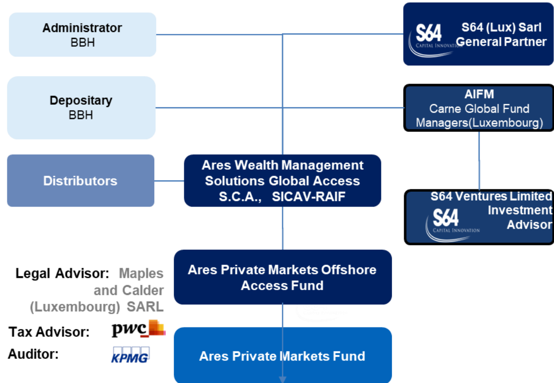
Structure Chart
